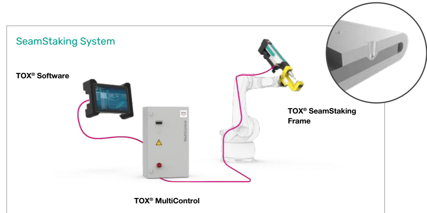
TOX® SeamStaking System as robot guided system.
