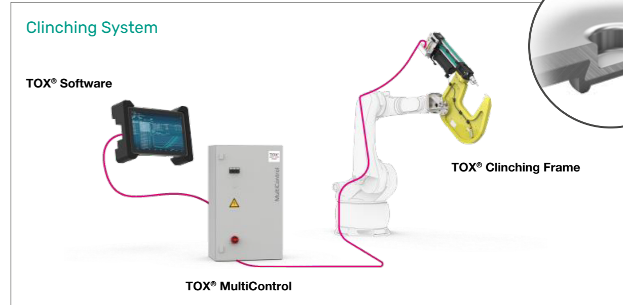
TOX® Clinching System as robot guided system. Also possible as stationary system.
